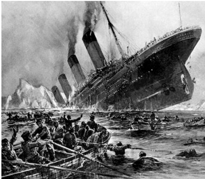
Titanic adathalmaz
